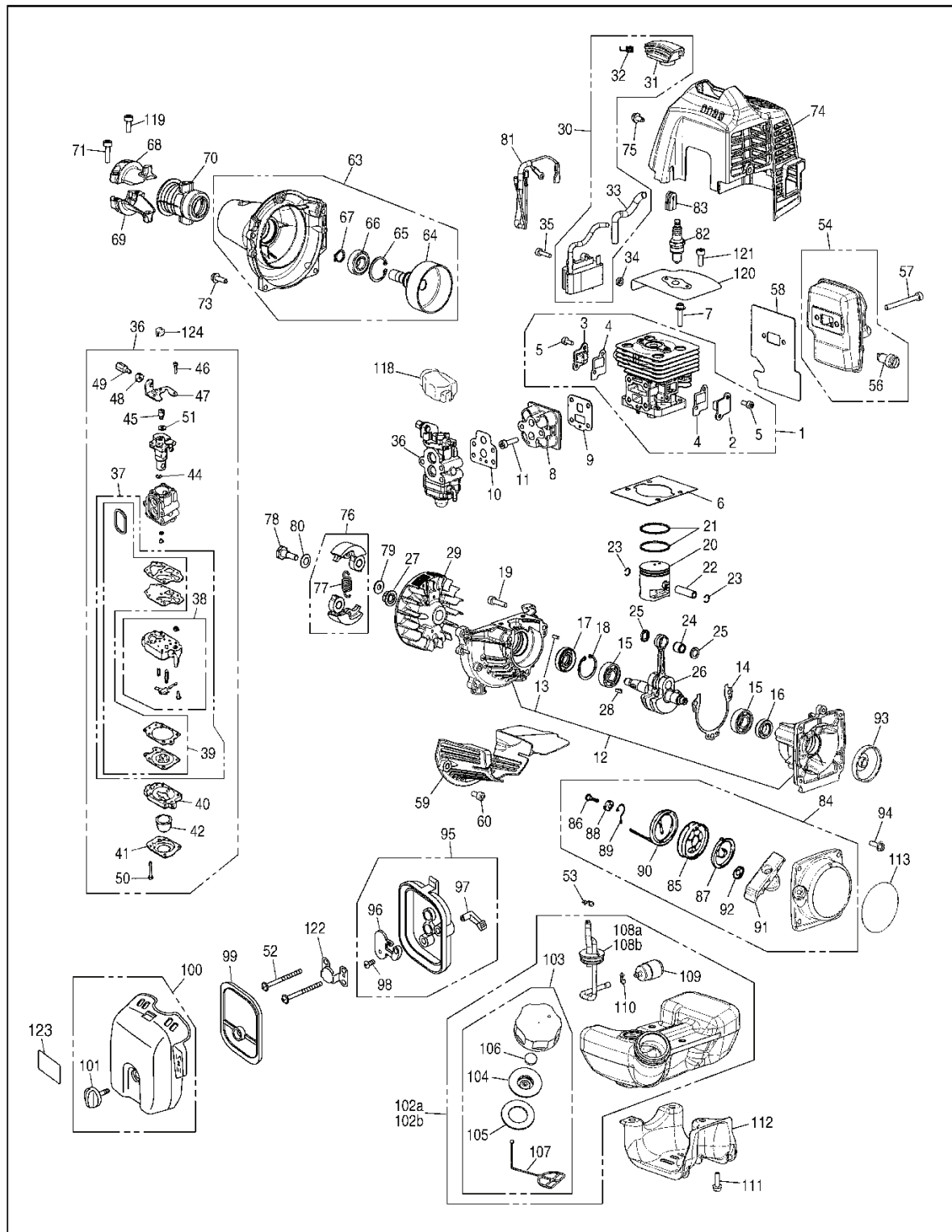
Fig.3 ENGINE UNIT
