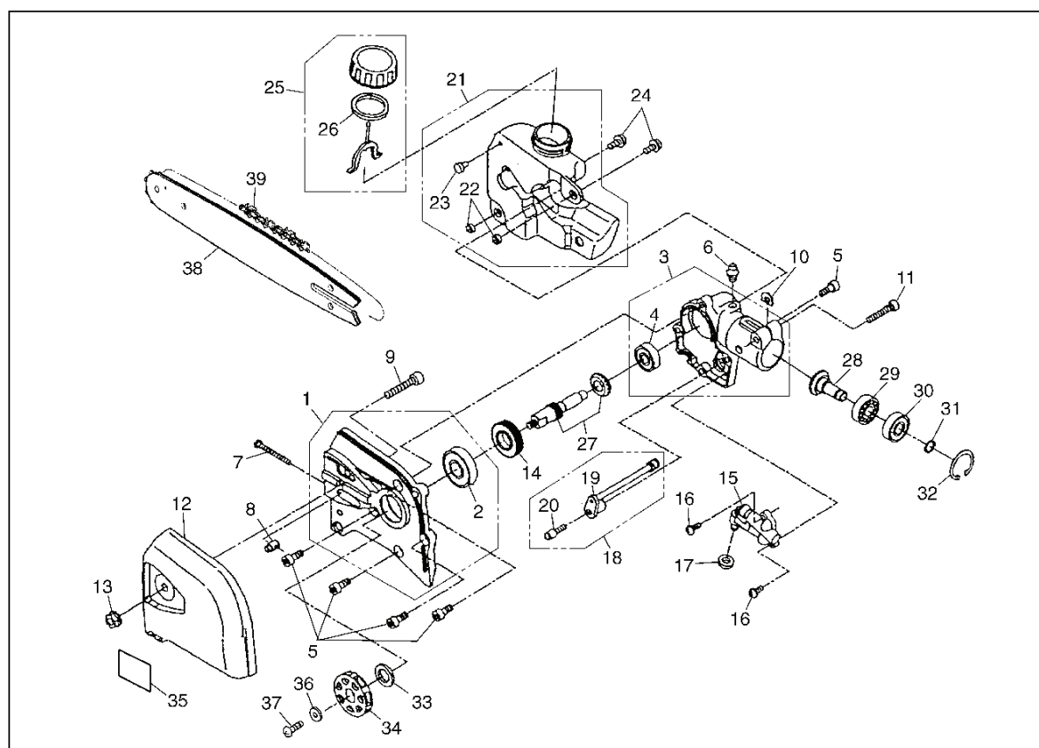
Fig.2 CUTTING UNIT
