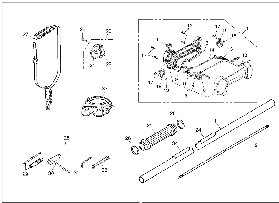
Fig.1 DRIVE UNIT
