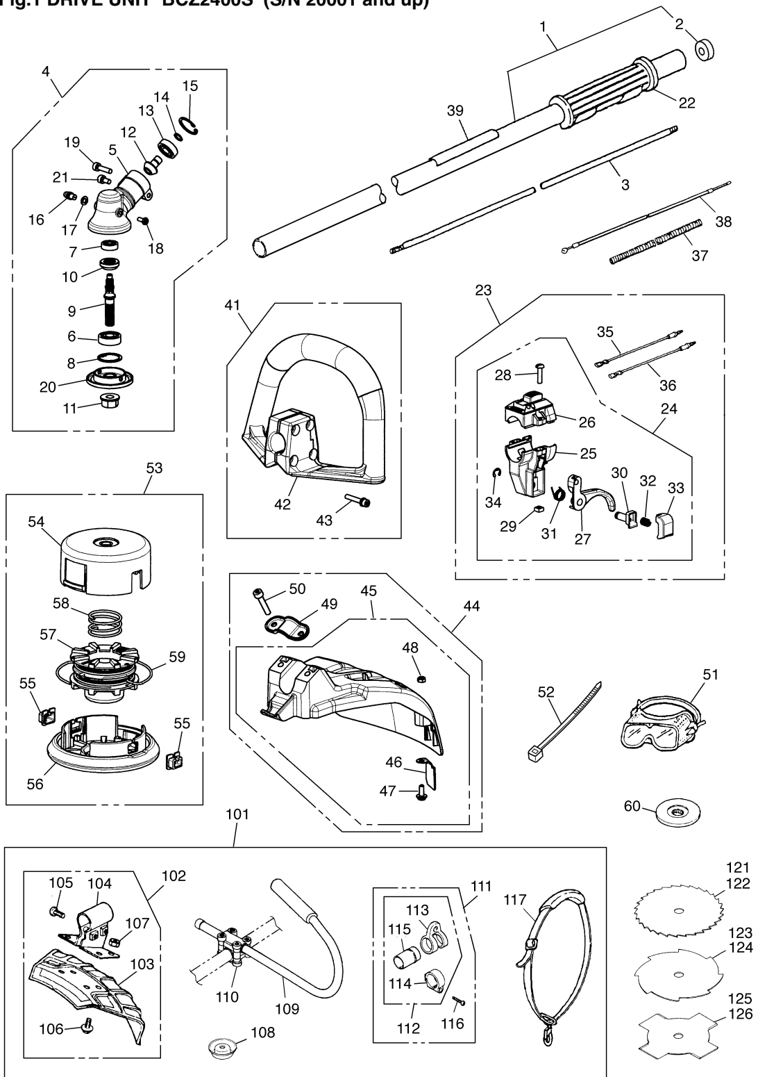
Fig.1 DRIVE UNIT BCZ2400S (S/N 2001 and up)
