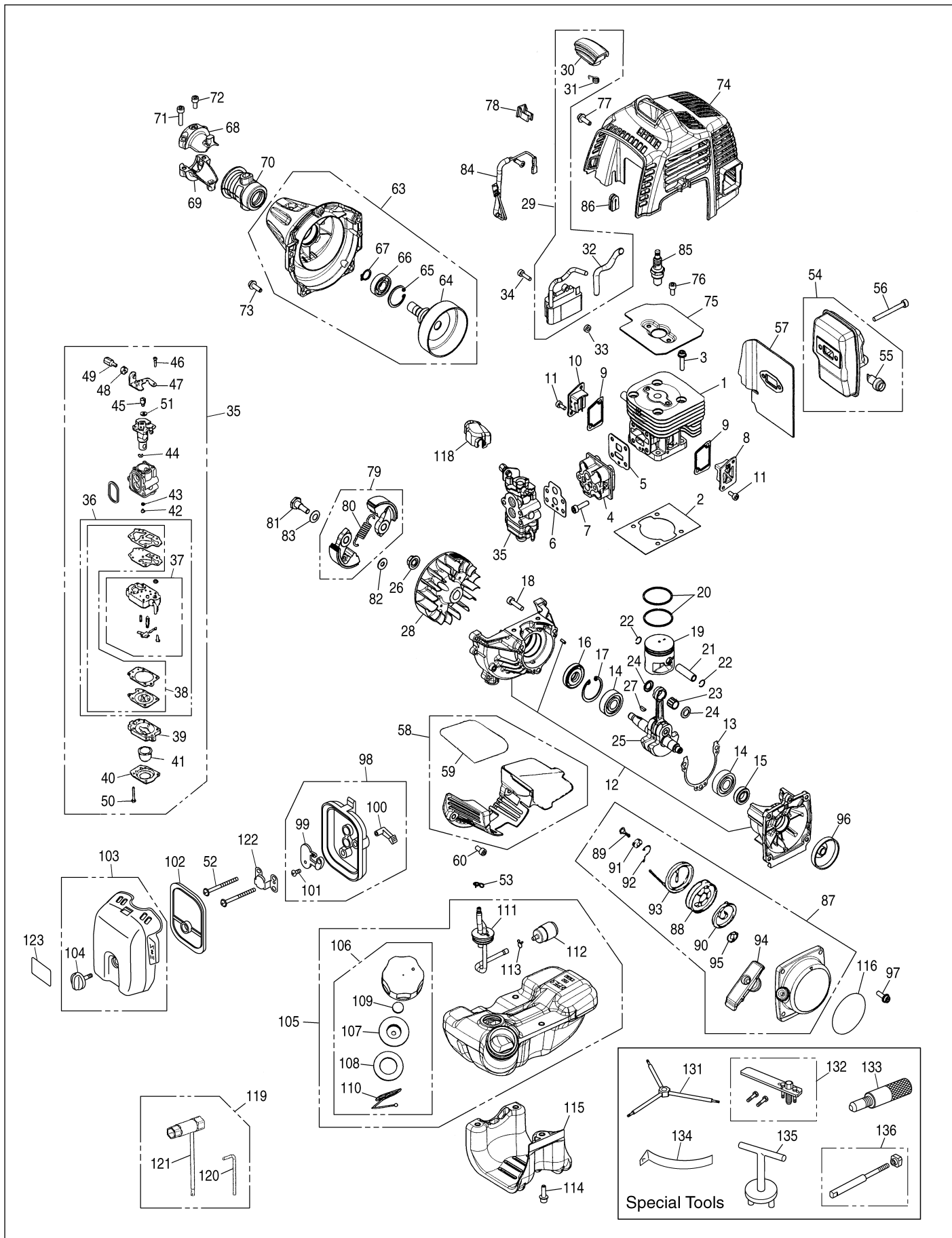
Fig.4 ENGINE UNIT
