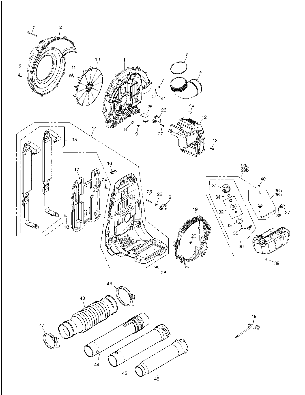
Fig.1 BLOWER GROUP
