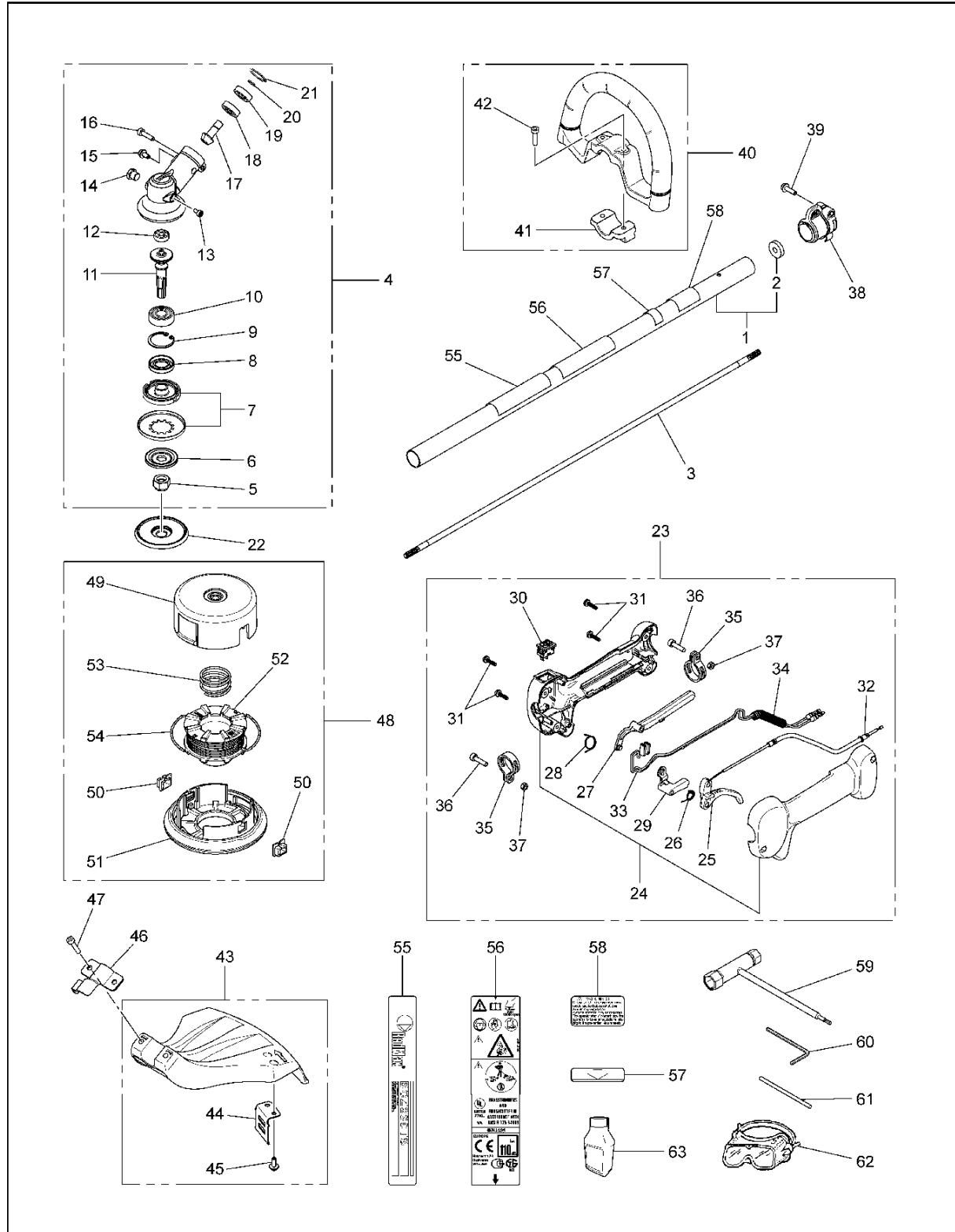
Fig.1 DRIVE UNIT
